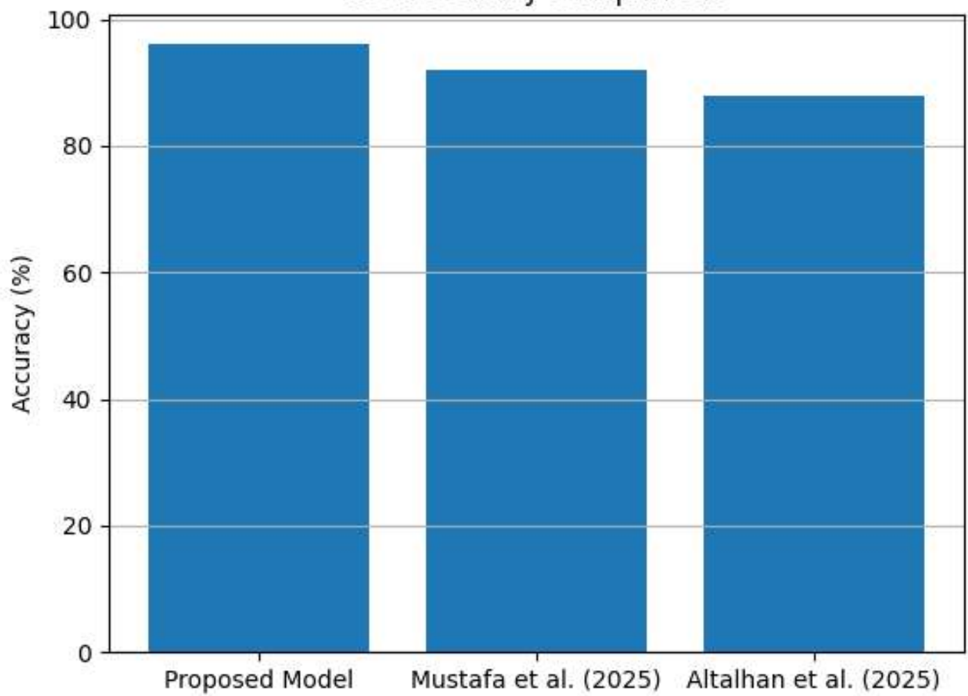
IDS Accuracy Comparison
